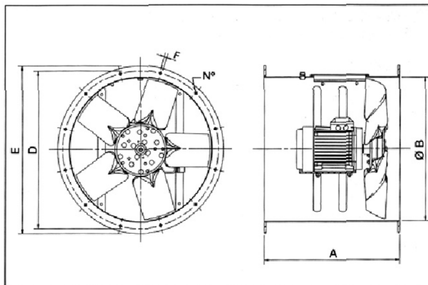
TGT-560 to TGT-1250 (long casing)
