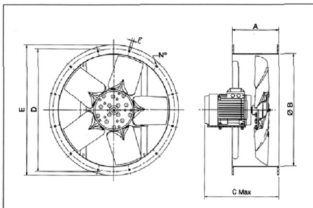
TGT-560 to TGT-1250 (short casing)
